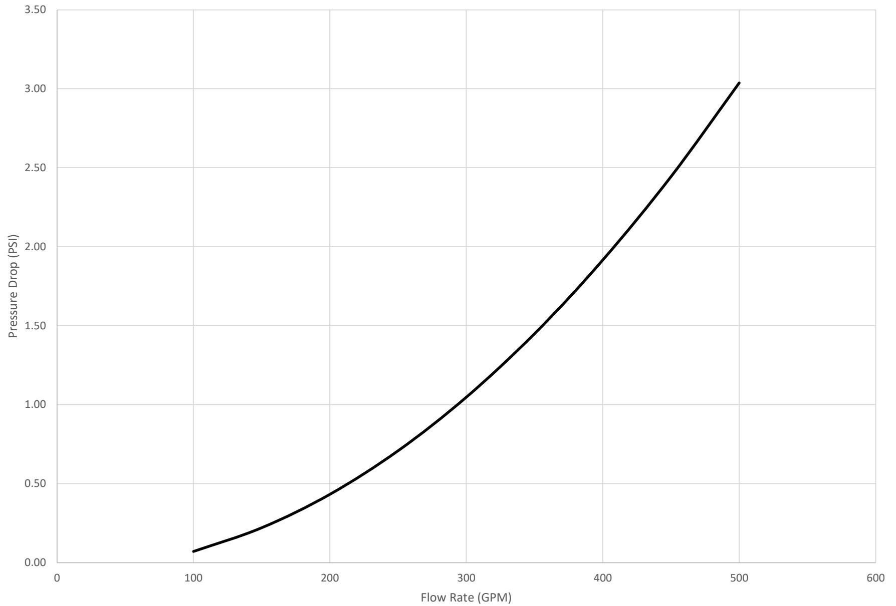
BMK4000 & BMK5000N Pressure Drop Chart
