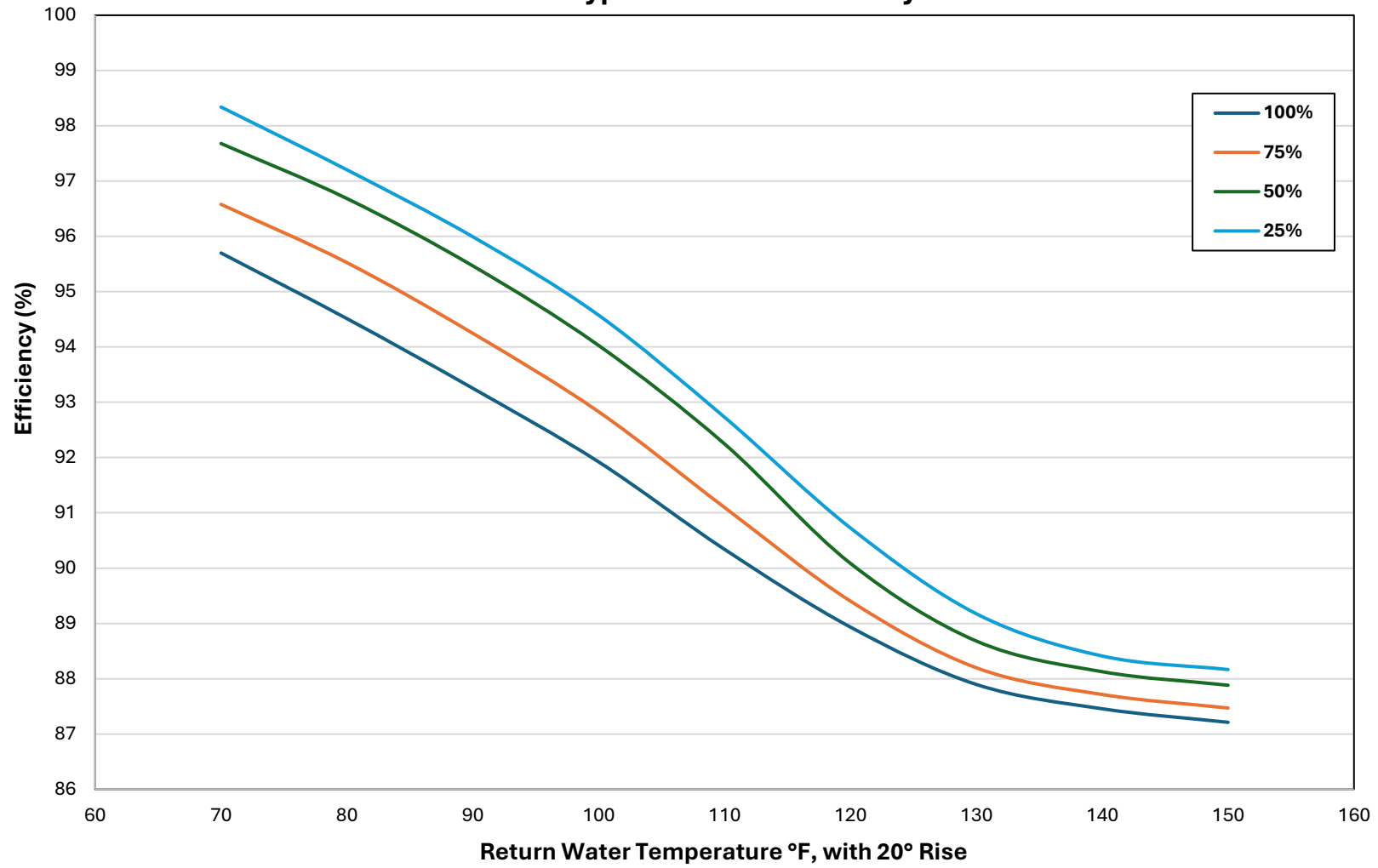
Typical MFC II Efficiency
