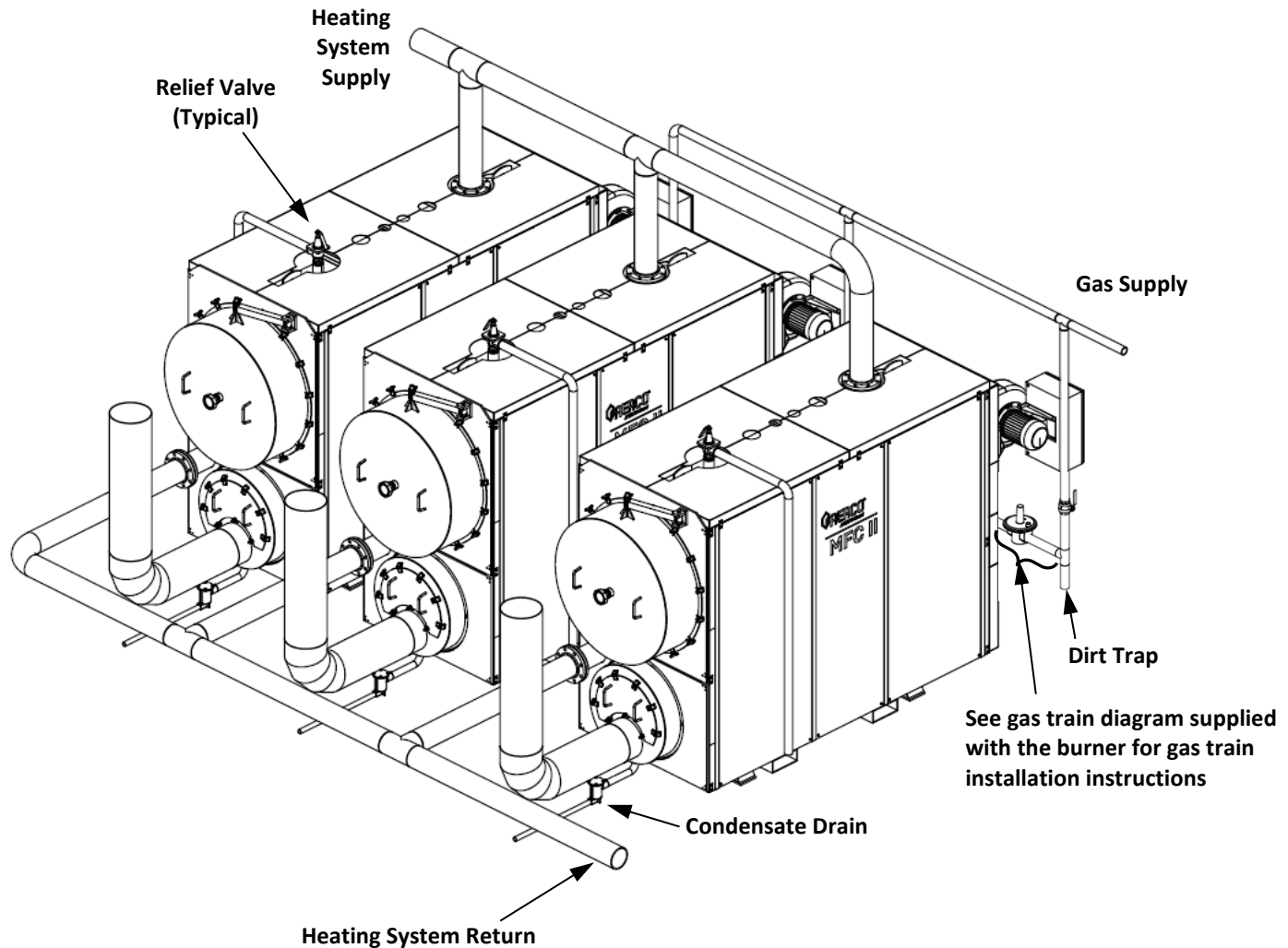
Diagram 2: Typical Multiple Boiler Manifold Construction
