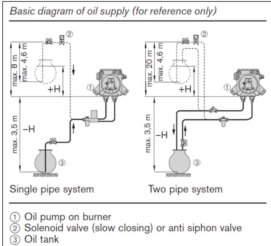
Diagram 4: Oil Fuel Supply Design and Function
