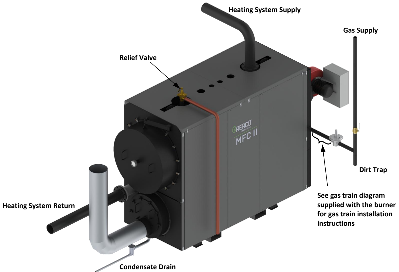
Diagram 1: Single Boiler Gas Pipe Connections
