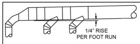
Figure 11-1: Connection of Unit at End of Vent Main
