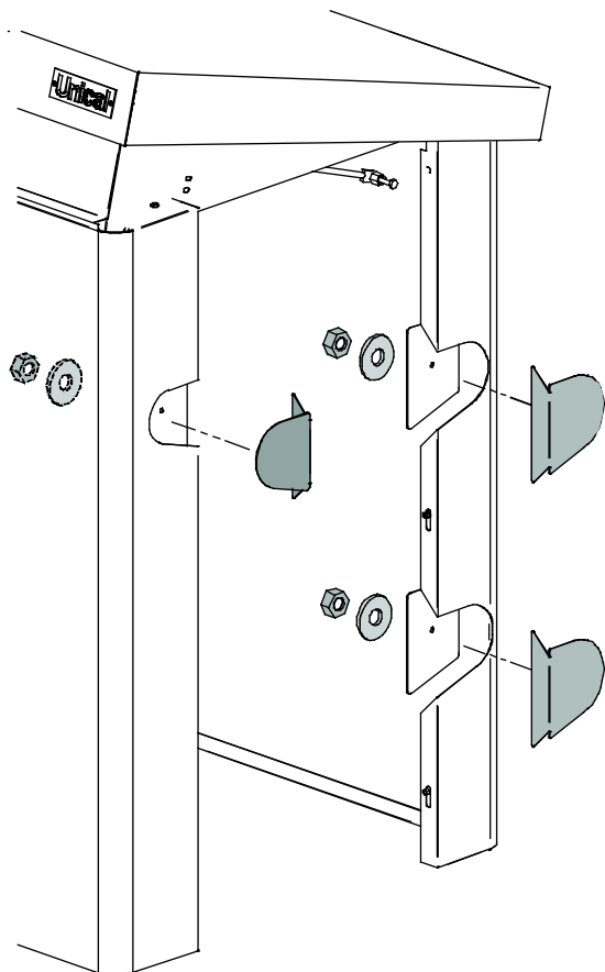
Figure 13: Caps and Plugs Used for Closing Up Vacated Gas and Hydraulic Connection Openings
