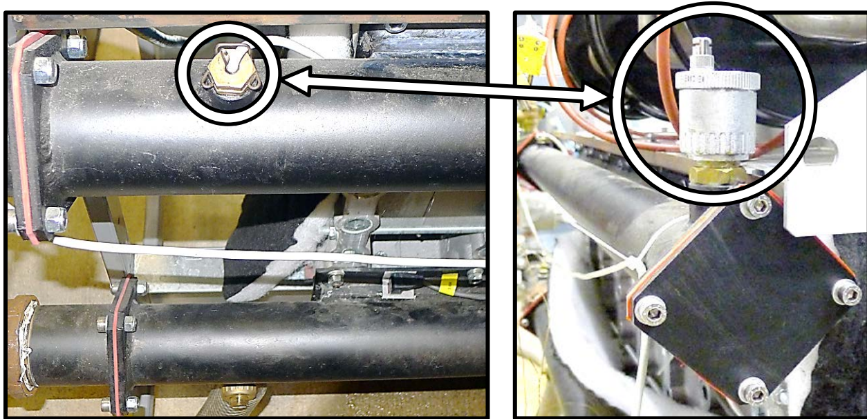
Figure 12: Reversing Boiler Sensor KF with Automatic Air Vent
