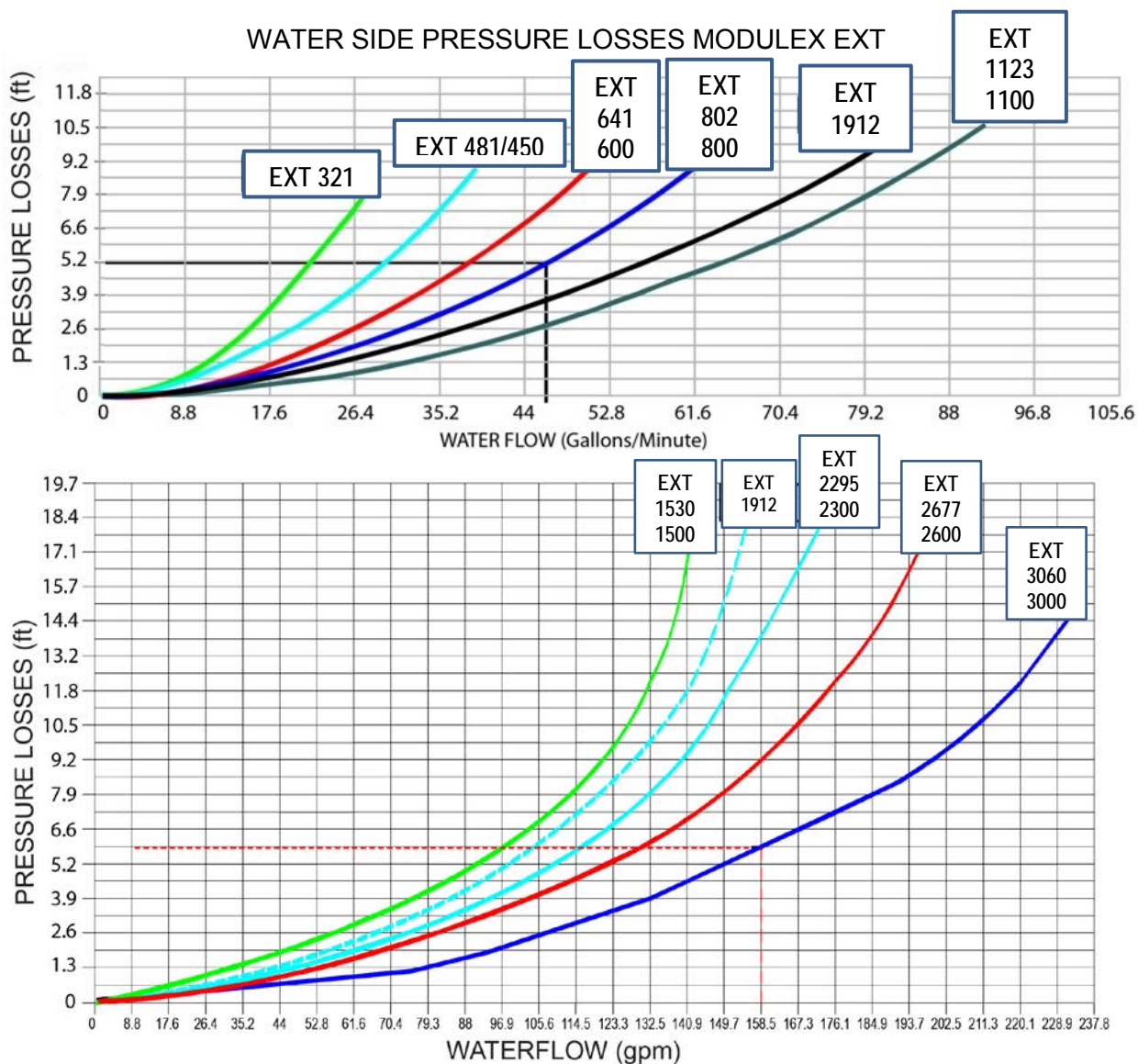
Figure 2: Water Side Pressure Loss Charts
