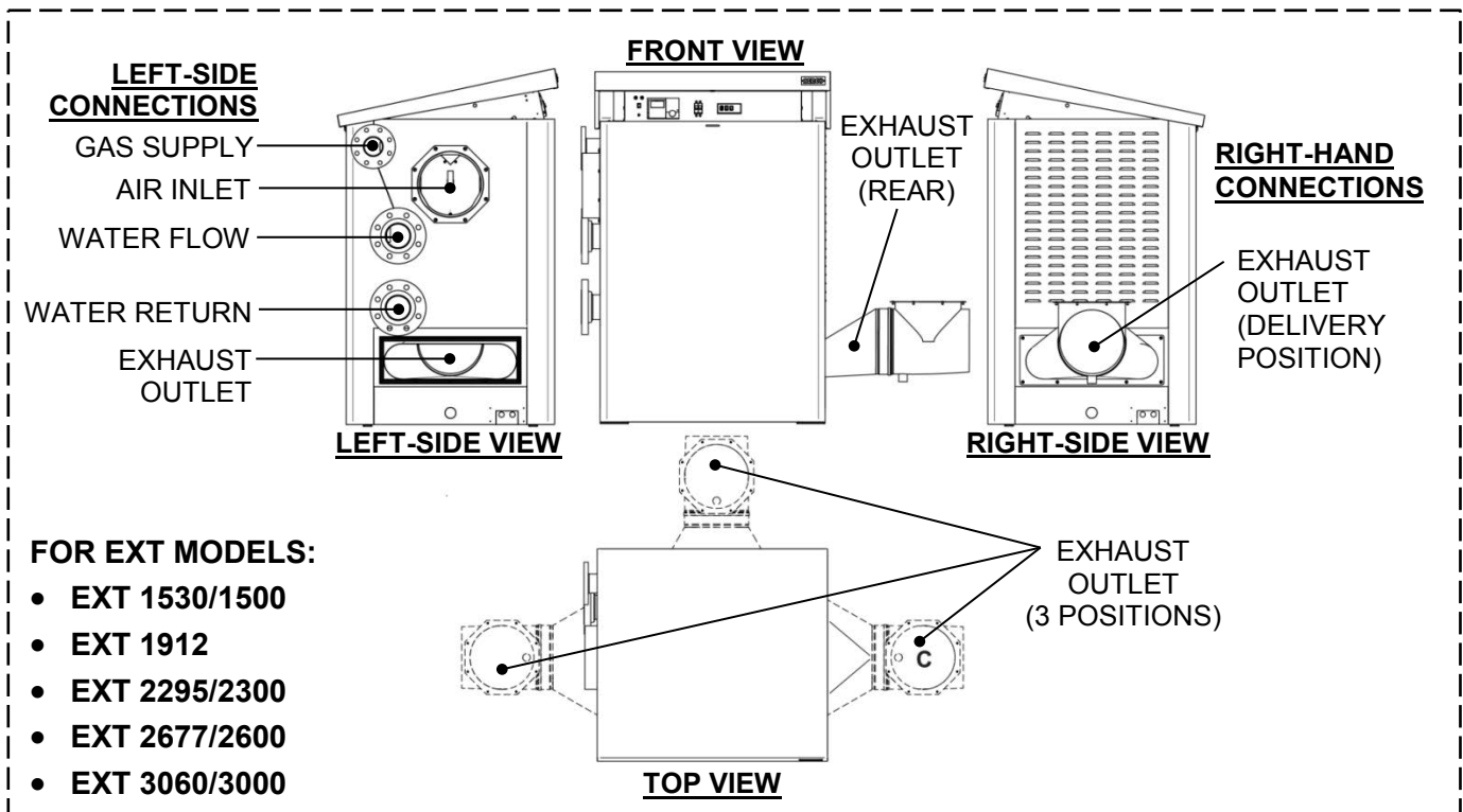
Figure 8: Locations for Left-Hand and Right-Hand Connections
