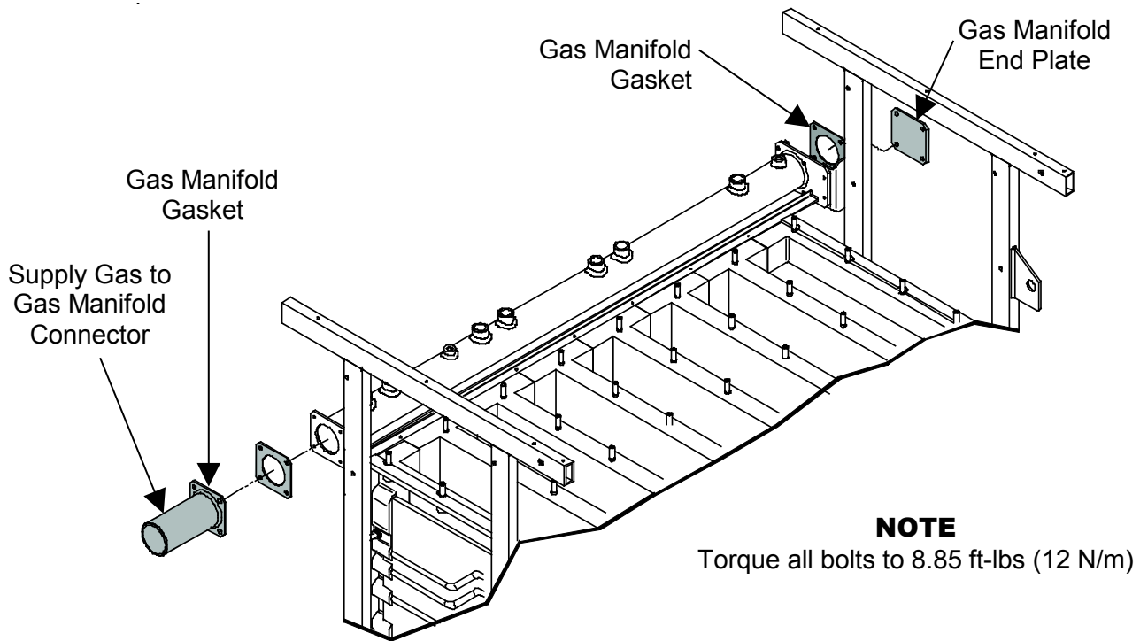
Figure 9: Reversing Gas Connections from RIGHT-HAND to LEFT-HAND for EXT 321, 481/450, 641, 802/800, 962, and 1123/1100
