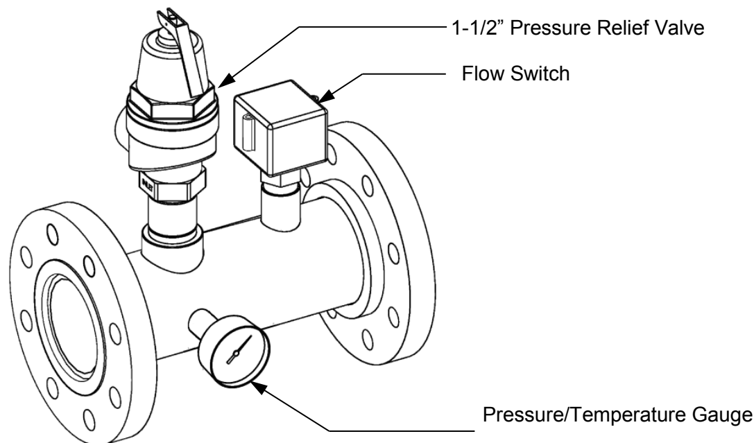
Figure 6: Manifold Assembly and Components for EXT 1530/1500 through EXT 3060/3000
