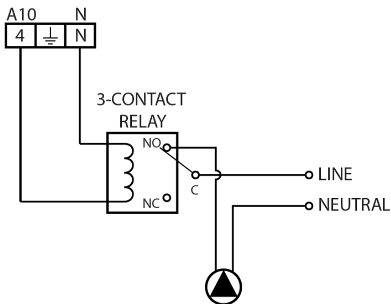
Figure 3: Electrical Connection of Primary Pump
