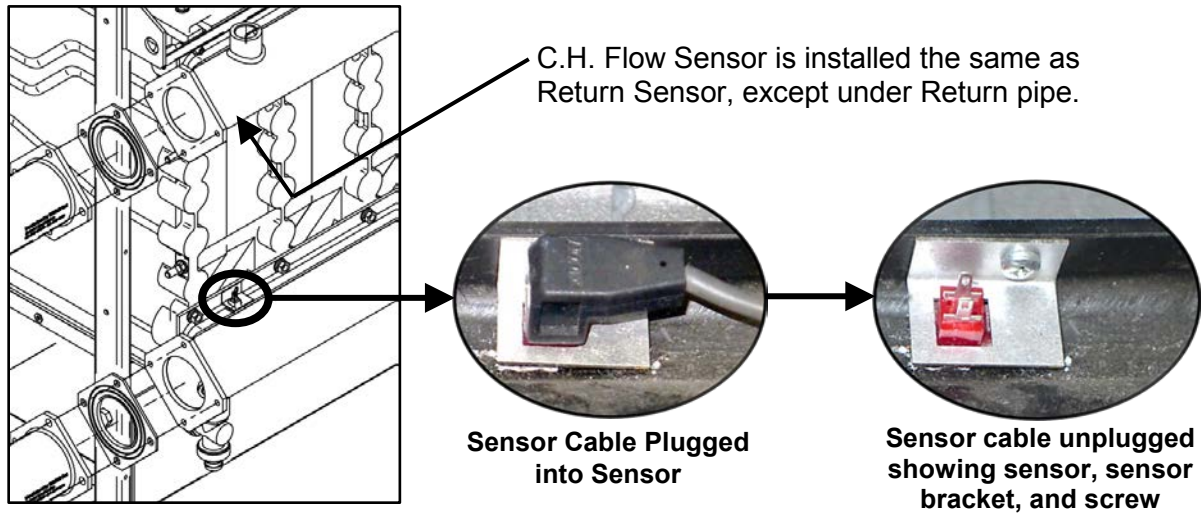
Figure 11: Reversing Flow and Return Temperature Sensors
