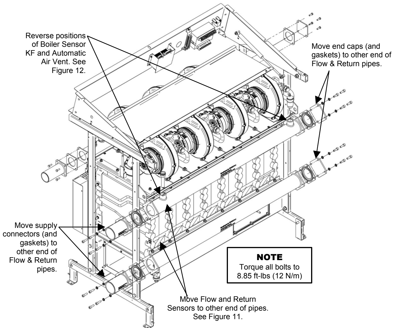
Figure 10: Reversing Cold/Hot Water Flow and Return Connections and Sensors from RIGHT HAND to LEFT HAND
