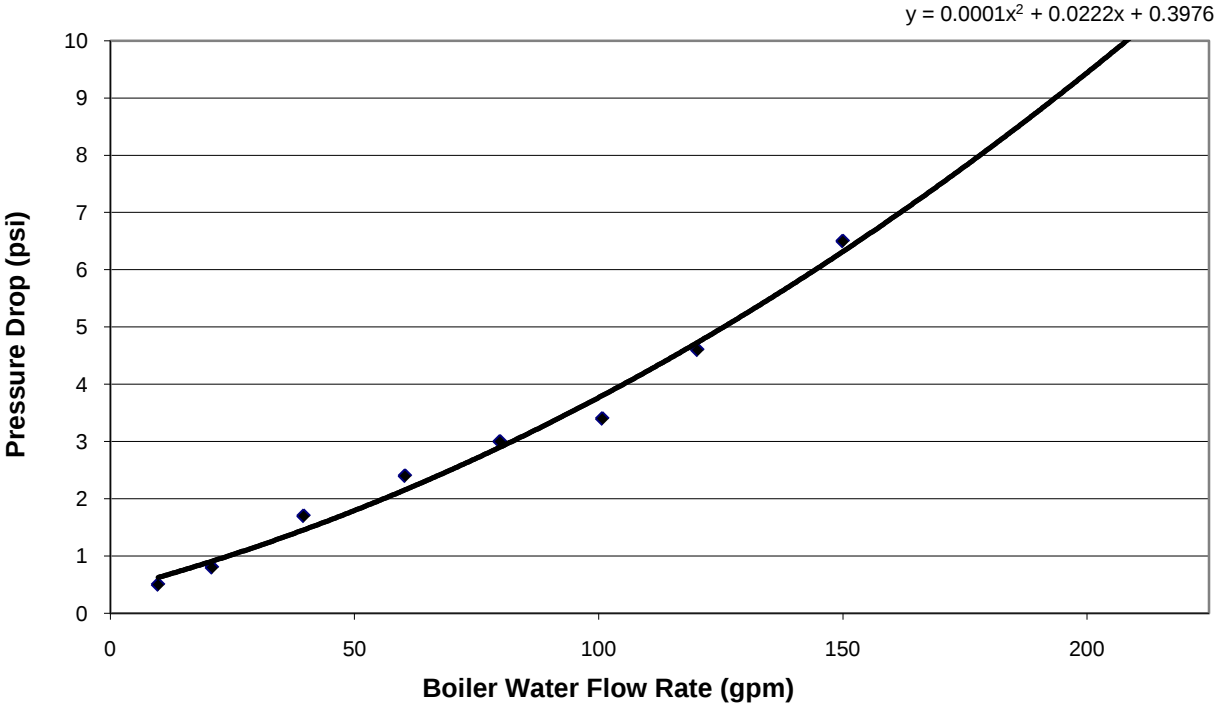
BMK 1.5MMBTU Boiler Waterside Pressure Drop
